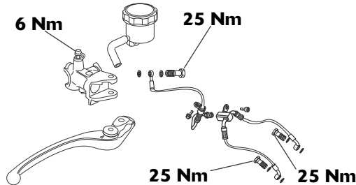
Front brakes from VIN 461332
