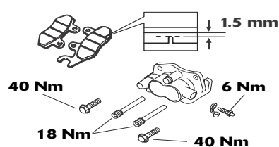
Rear brakes from VIN 461332
