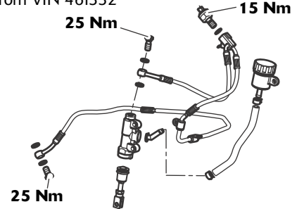
Rear brakes from VIN 461332
